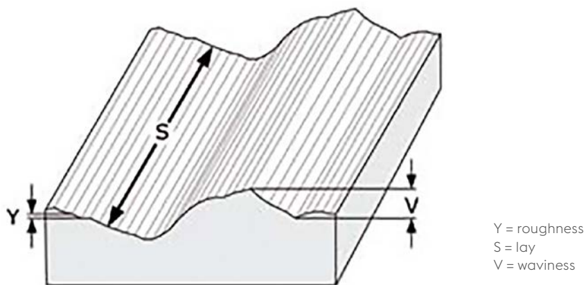
Surface roughness
