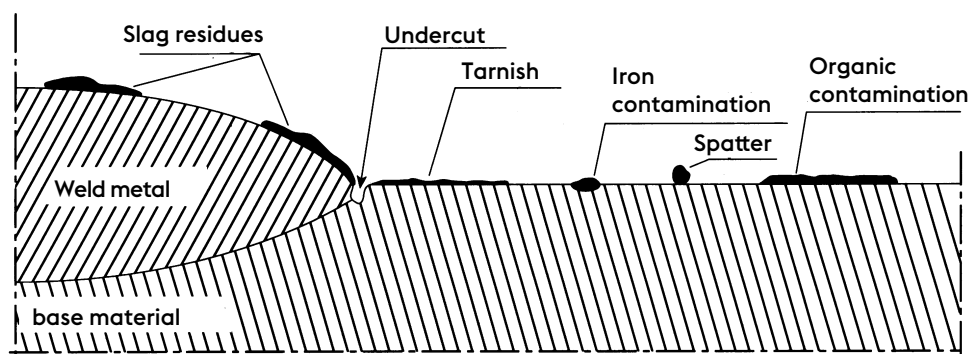
Surface defects
